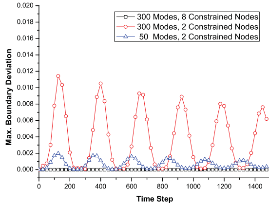
Figure 3. Boundary deviation comparisons with different number of modes and boundary constraint nodes.
