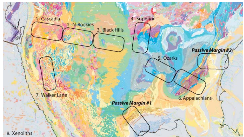
Fig. 1. The GeoSwath focus areas numbered 1–7 plus xenolith database [Tikoff et al. , 2006] placed on the 2005 Geologic Map of North America [Reed et al. , 2005]. We have deleted the coastline and emboldened the 3000-meter isobath to stress the point that continental geology does not stop at the coastline. Additional boxes labeled Passive Margin #1 and Passive Margin #2 are just two of many possible candidate focus areas where the U.S. passive continental margins could be studied. Figure modifications thanks to E. A. Hinz.
