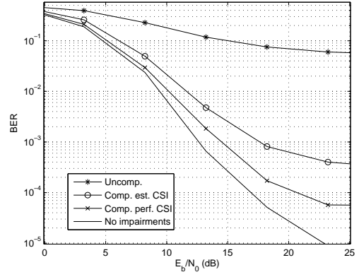
Fig. 10. Performance of 64-QAM SFBC-OFDM scheme with channel estimation (FI I/Q imbalance \alpha_r = \alpha_t = 0.5 dB, \theta_r = \theta_t = 5^\circ , \tilde{\xi}_r^I(n) = \tilde{\xi}_t^I(n) = \delta(n) + 0.1\delta(n-1) , \tilde{\xi}_r^Q(n) = \tilde{\xi}_t^Q(n) = \delta(n) - 0.1\delta(n-1) , Doppler=2% of sub-carrier spacing, CFO=1%)
