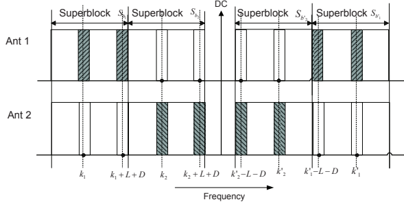
(a) SFBC-OFDM
