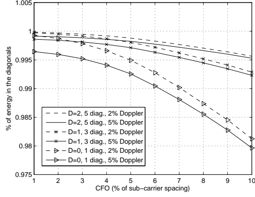
Fig. 4. Energy distribution in the diagonals of the channel matrix for different Doppler values and residual CFO levels
