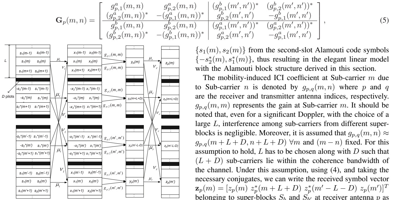
Fig. 2. Proposed super-block structure for Alamouti SFBC-OFDM
