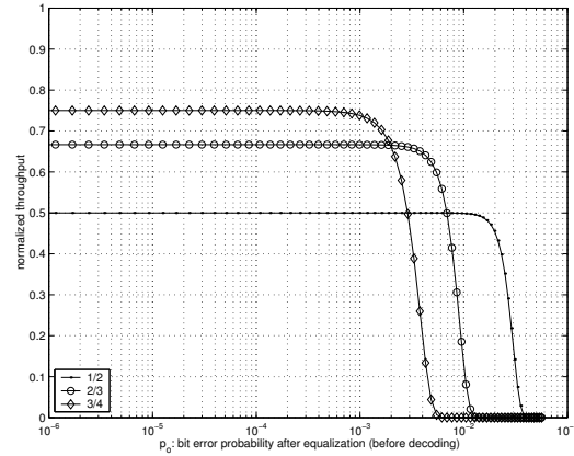
Figure 2: Theoretical normalized throughput
