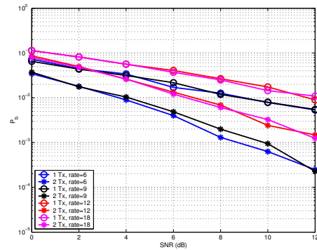
Figure 1: BER for channel “A”
