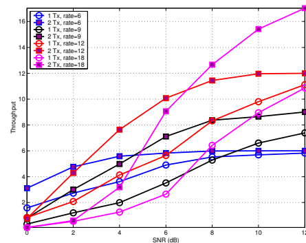
Figure 3: Throughput for HiperLan/2 channel “A”
