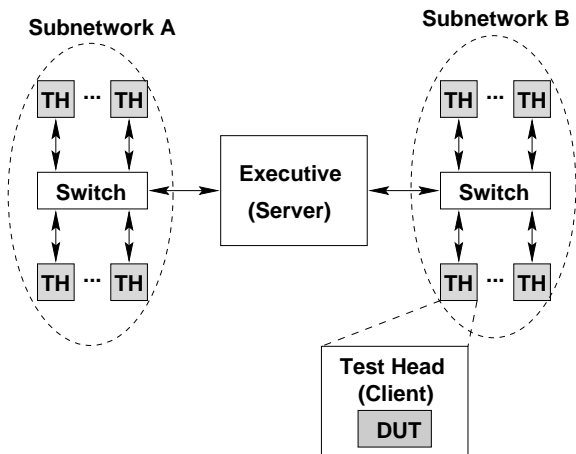
Fig. 3. TAN Architecture
