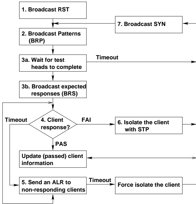
Fig. 6. FSM of TAN Protocol Execution
