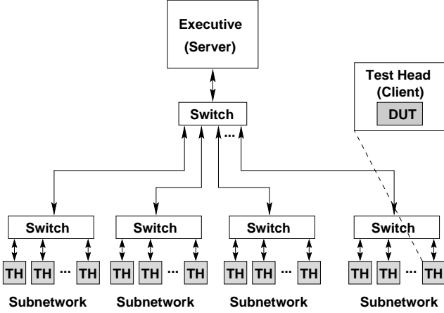
Fig. 8. Infinite-pin configuration
