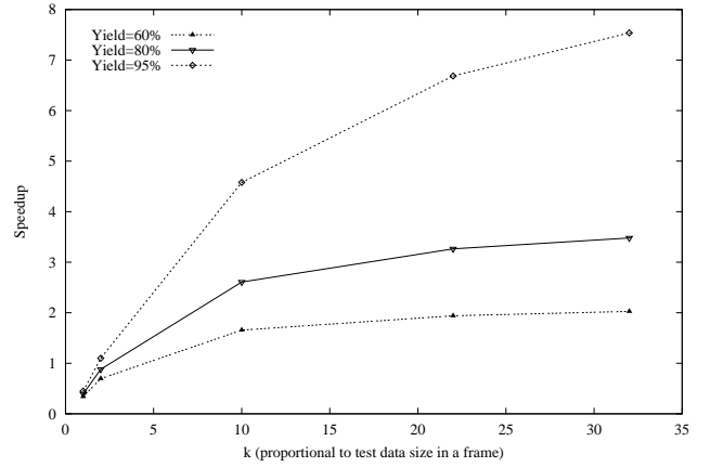
Fig. 10. Plot of speedup vs k
