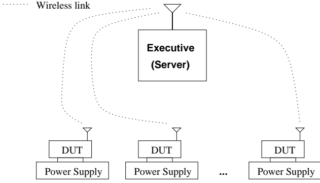
Fig. 7. Zero-pin configuration
