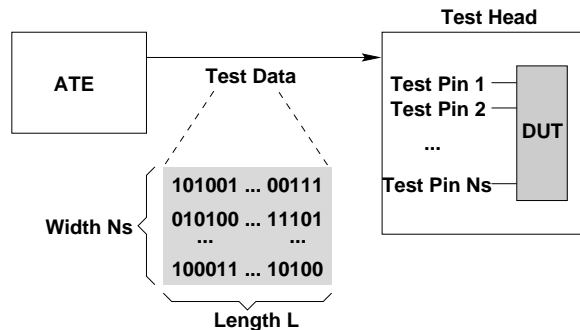
Fig. 2. Test model
