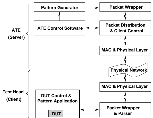
Fig. 4. Client and Server architecture
