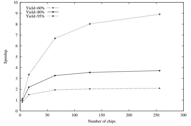
Fig. 9. Plot of speedup vs number of chips under test
