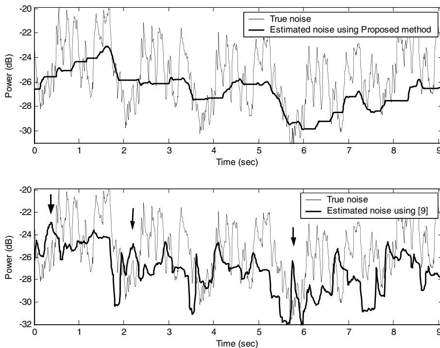
Fig. 6. Top panel: Plot of true noise spectrum and estimated noise spectrum using the proposed method for a noisy speech signal (5 dB SNR) at f = 250 Hz. Bottom panel: Plot of true noise spectrum and estimated noise spectrum using (Doblinger, 1995). Arrows indicate regions where noise is overestimated.
