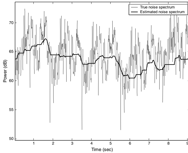
Fig. 4. Plot of true noise spectrum and the estimated noise spectrum using our proposed method for a speech degraded by babble noise at 5 dB SNR and single frequency f = 250 Hz.
