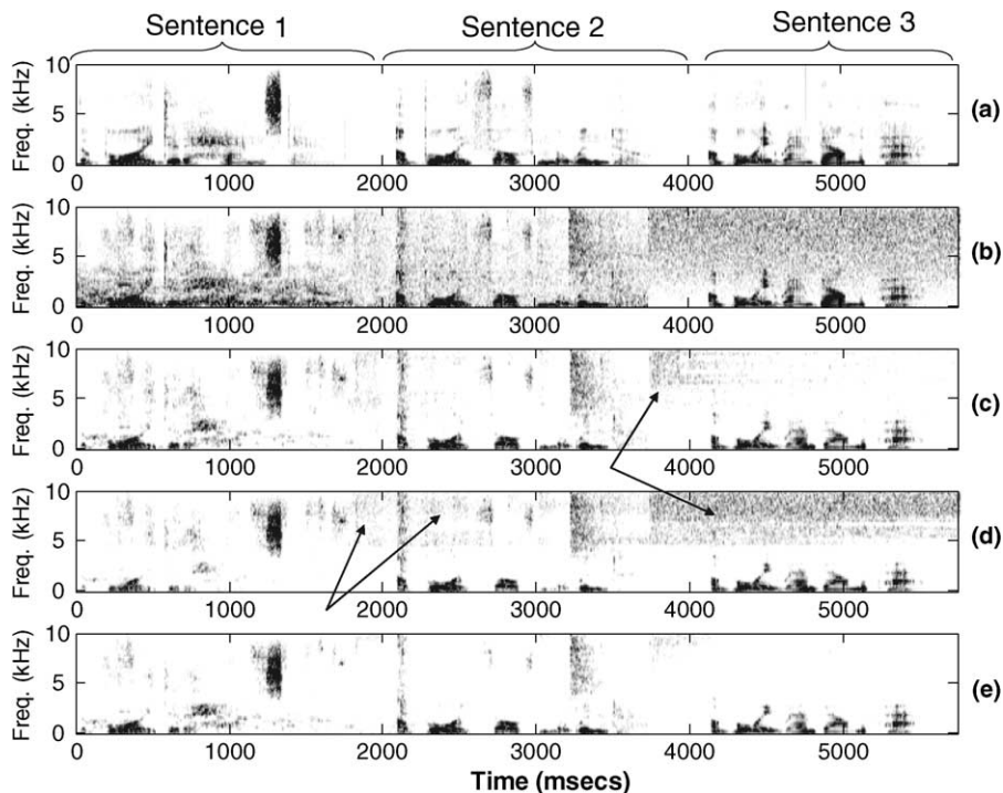
Fig. 8. Spectrograms of speech enhanced using Martin's (2001) noise-estimation method (panel c), Cohen's method (Cohen (2003)) (panel d) and the proposed noise-estimation method (panel e). Spectrograms of the clean and noisy speech signals are given in panels (a) and (b) respectively. Arrows in panels (c) and (d) at t > 3.8 s show the presence of residual noise due partly to the inability of the noise-estimation algorithms to track the sudden appearance of high-frequency noise in the last sentence (sentence 3). In contrast, as shown in panel (e), the residual noise is greatly reduced with the proposed noise-estimation algorithm.
