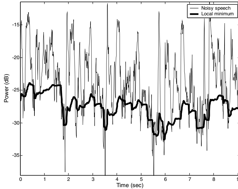
Fig. 2. Plot of noisy speech power spectrum and local minimum using (3) for a speech degraded by babble noise at 5 dB SNR at frequency bin k = 5 .
