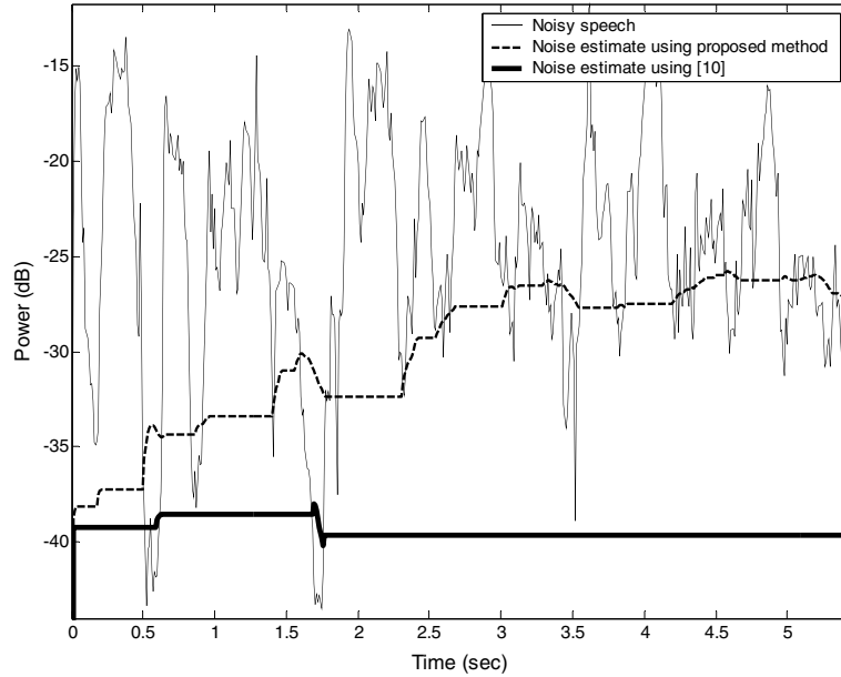
Fig. 7. Comparison of estimated noise spectrum ( f = 500 Hz) of proposed method (dashed line) with that of Hirsch and Ehrlicher (1995) (solid line) for a noisy speech of SNR 20 dB ( t < 1.8 s) followed by a noisy speech of SNR 5 dB ( t > 1.8 s).
