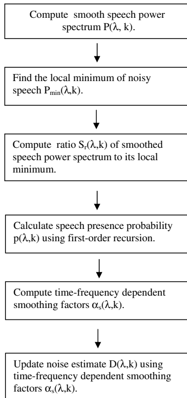
Fig. 1. Flow diagram of proposed noise-estimation algorithm.
