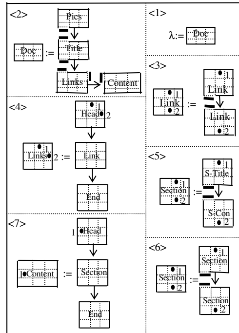
Figure 7 Graph grammar
