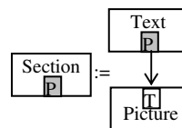
Figure 1 A production in RGG
