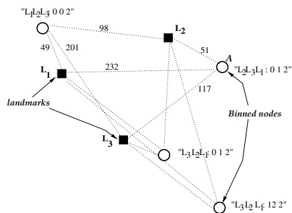
Fig. 1. Distributed binning
