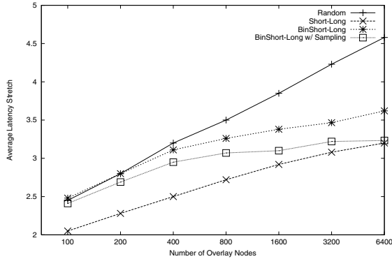
Fig. 9. Unstructured Overlays; TS-10K; #levels=1; #landmarks=12
