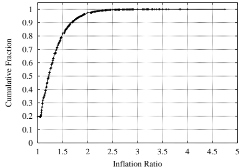
Fig. 4. Cumulative distribution of inflation ratio
