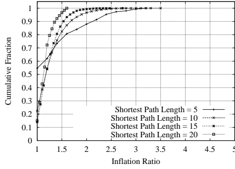
Fig. 6. Cumulative distribution of inflation ratio by path length
