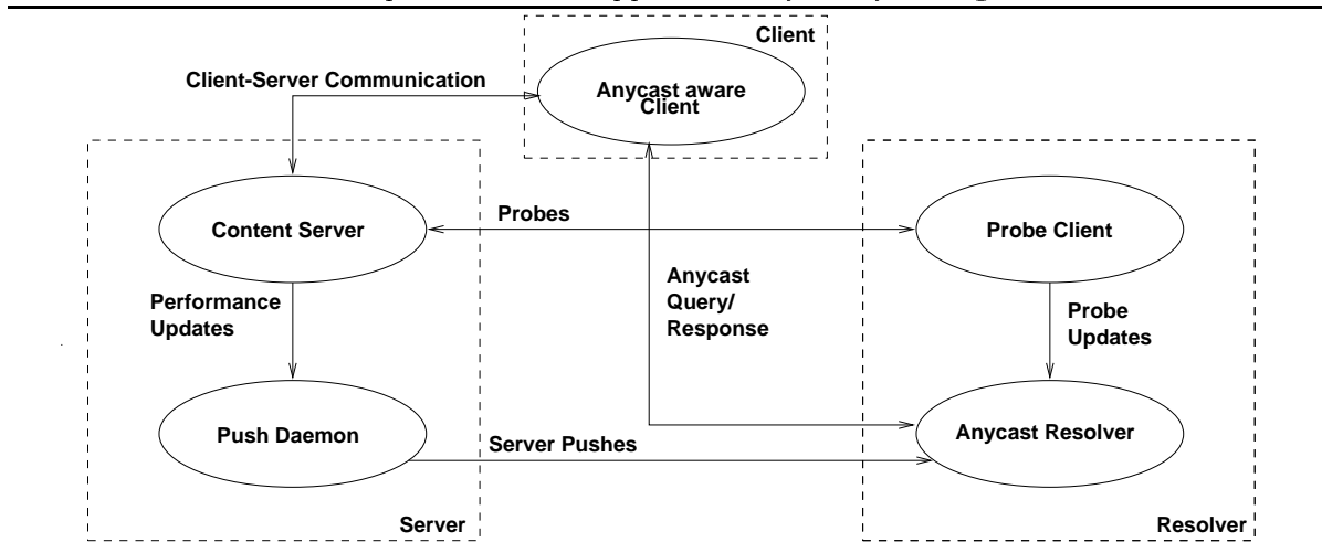
FIGURE 4 Software components of the application-layer anycasting architecture
