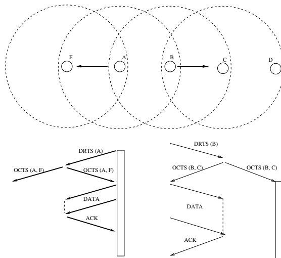
Fig. 3. Another Example of using Directional MAC Scheme 1
