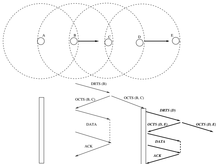
Fig. 2. Example of using a Directional MAC Scheme 1: This figure uses notation similar to Figure 1. Letters in parentheses, such as DRTS(B) or OCTS(B,C), denote the physical location information included in the message. The white box below node D denotes that node D may transmit to node E in the corresponding duration, unlike when using omnidirectional antennas.
