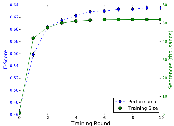
Figure 2: Learning and training set size curves.
