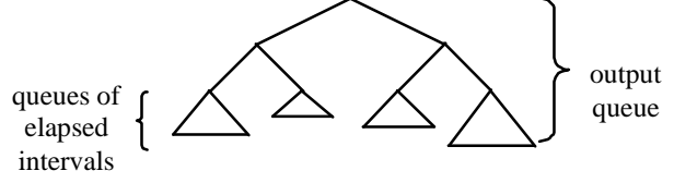
Fig. 4. Output queue of scheduler with eligibility times.
