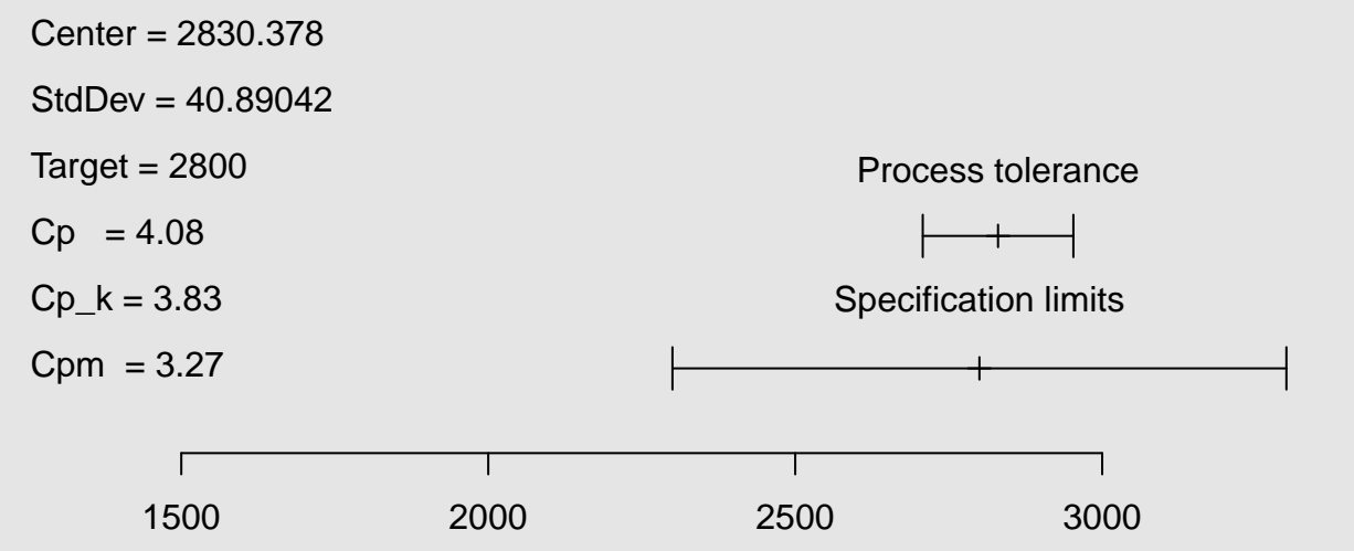
Capability plot
