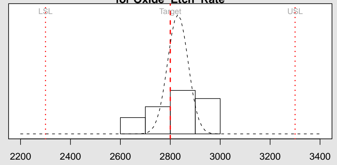
Process Capability Analysis for Oxide Etch Rate
