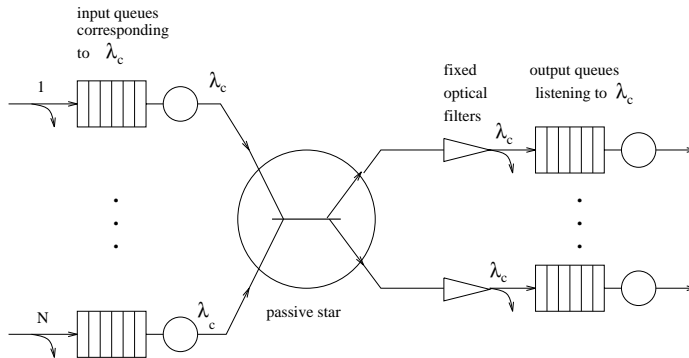
Figure 3: Queueing sub-network for wavelength \lambda_c
