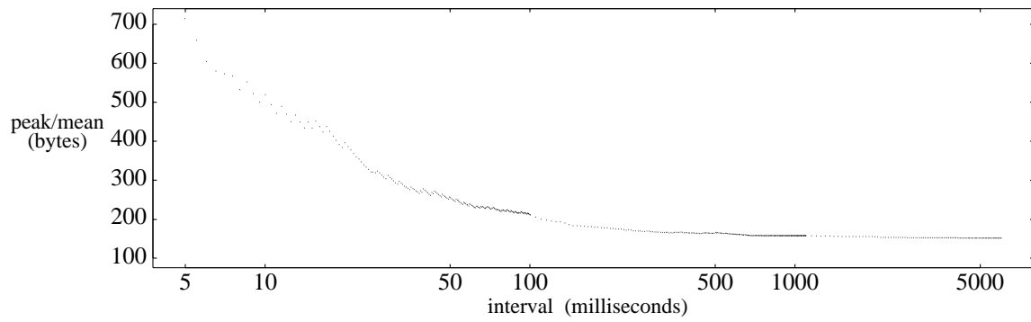
Figure 3.2.2: Peak to mean ratio for external traffic 307 hours of external traffic
