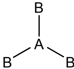
Trigonal planar
