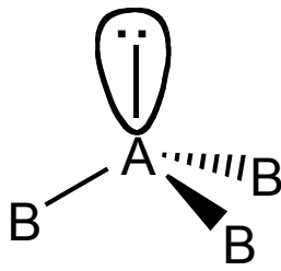
Trigonal pyramidal
