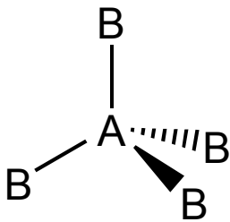
Tetrahedral
